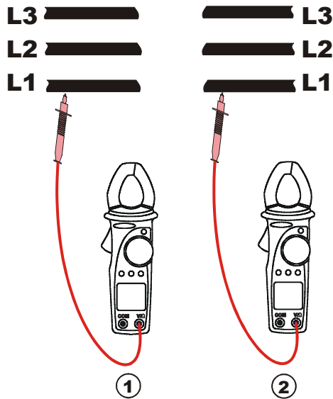
Fig. 14: phase detection
