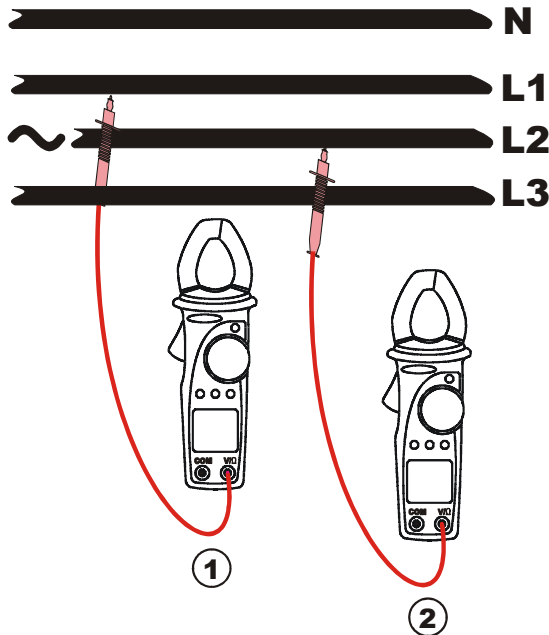
Fig. 12: phase rotation detection
