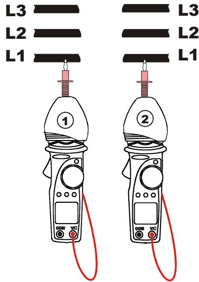
Fig. 15: phase detection with rubber cup
