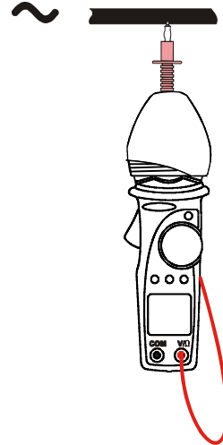
Fig. 17: Voltage detection with rubber cup
