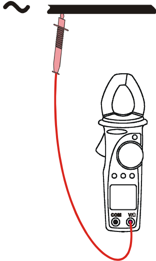
Fig. 16: Voltage detection
