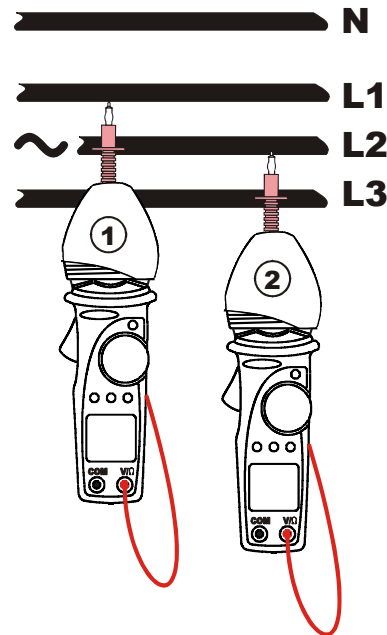
Fig. 13: phase rotation detection with rubber cup
